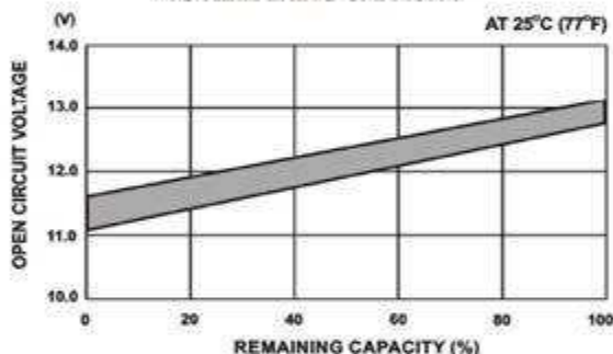
OPEN CIRCUIT VOLTAGE VS REMAINING CAPACITY
