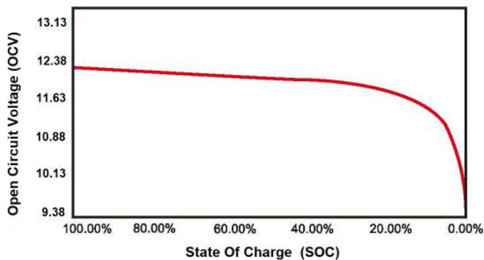
12.8V State Of Charge vs Open Circuit Voltage
